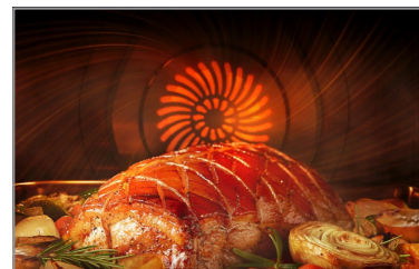
Convection véritable
